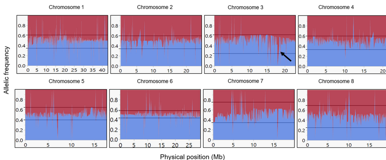
FIGURE 3 | Allelic frequency among the F1 population. Allelic frequency of the heterozygous allele in the F1 population for each marker. Blue line indicates the P. arabica allelic incidence, and red line indicates the U.E.F. allelic incidence. X-axis is the physical position in Mb, and y-axis represents the allelic ratio (from 0 to 1). Black arrow in chromosome 3 represents an example of unexpected deviated region ("hot spot"). References lines presented the "tolerance interval" limits.
