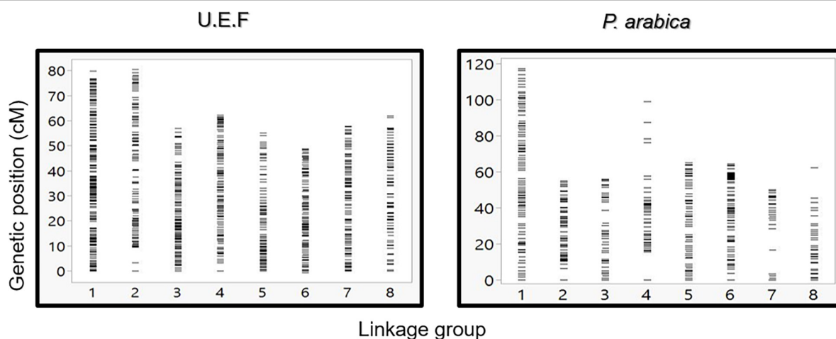
FIGURE 4 | Graphic presentation of markers density and distribution along the eight linkage groups. Comparison between U.E.F. map (left graph) and P. arabica map (right graph). Each horizontal line represents a single marker.
