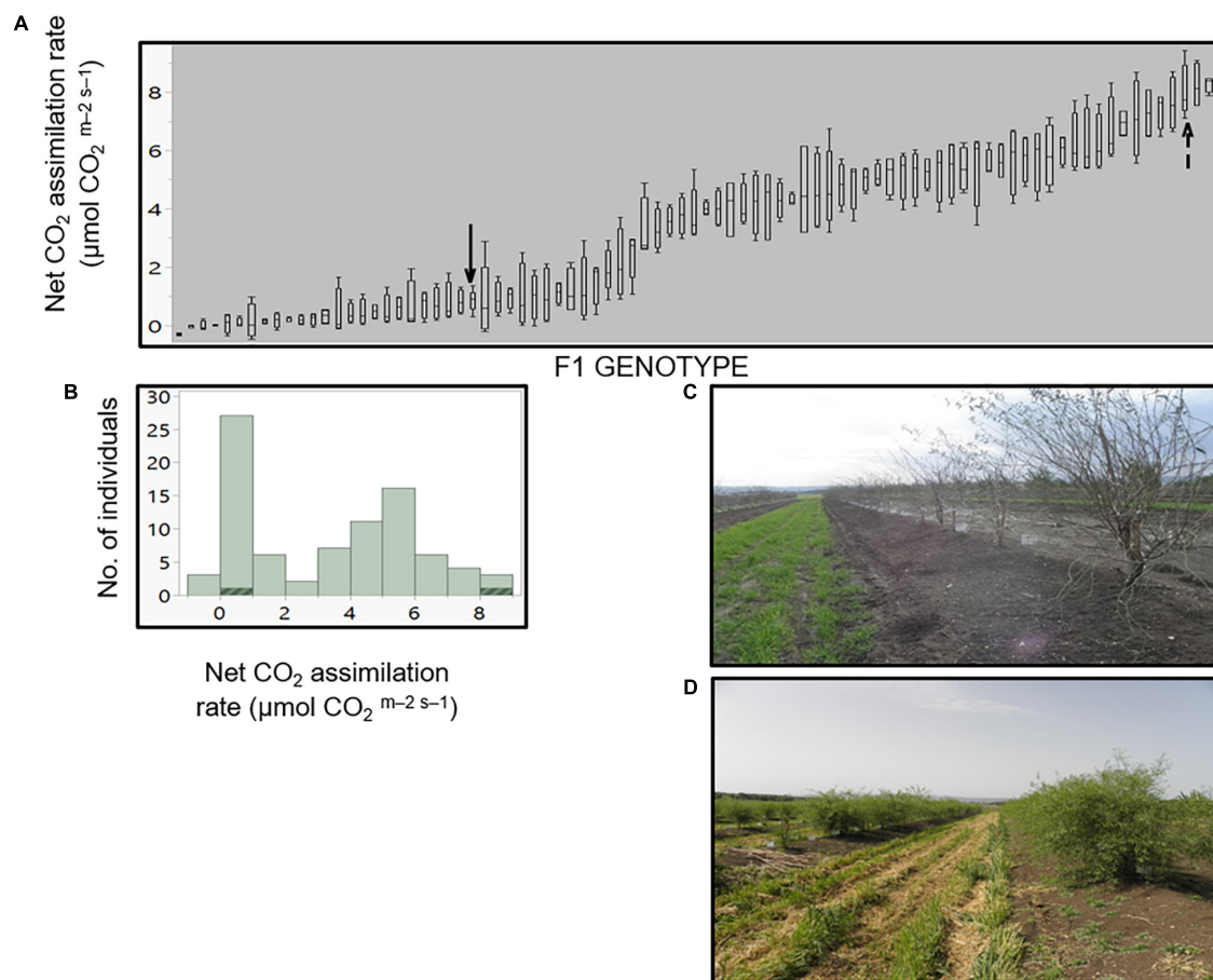
FIGURE 2 | Stem photosynthetic capability (SPC) in the F1 progeny. Levels of net CO 2 assimilation for each offspring (A). Each box plot presents the average of four stems ( n = 4 ). The F1 progeny parents, P. arabica and U.E.F. are marked by dashed arrow and simple arrow, respectively. Distribution histogram of the same data is presented in (B), while parents' data are highlighted. Measurements were conducted during February 2020, while the trees were dormant. Representative pictures of the F1 population while dormant (C) in February, and during the vegetative phase in April (D).
